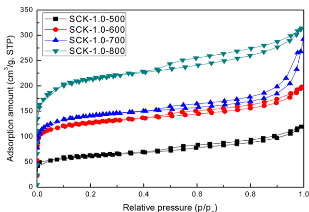
Fig. 3. Nitrogen adsorption-desorption isotherms of SCK at different activation temperatures.
